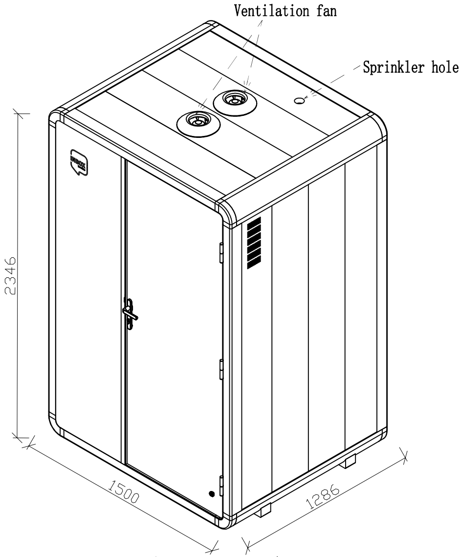
Axonometric drawing
