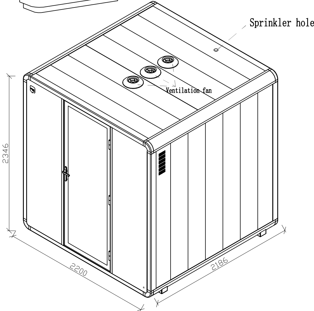
Axonometric drawing
