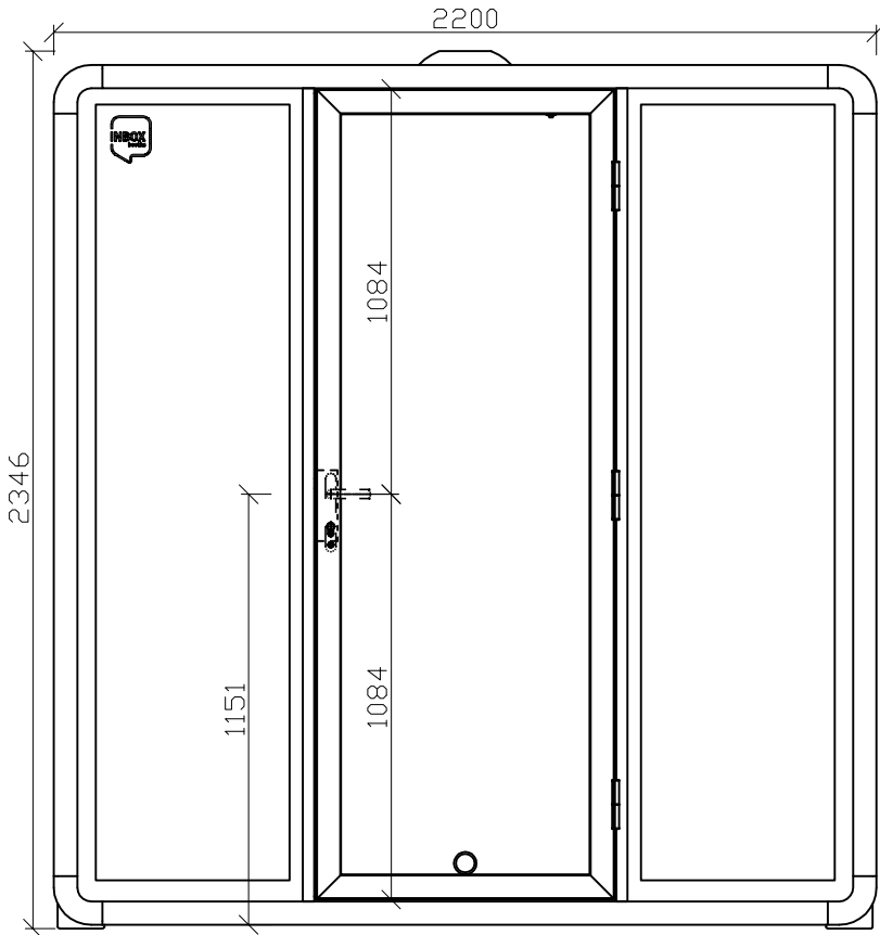
Front view
