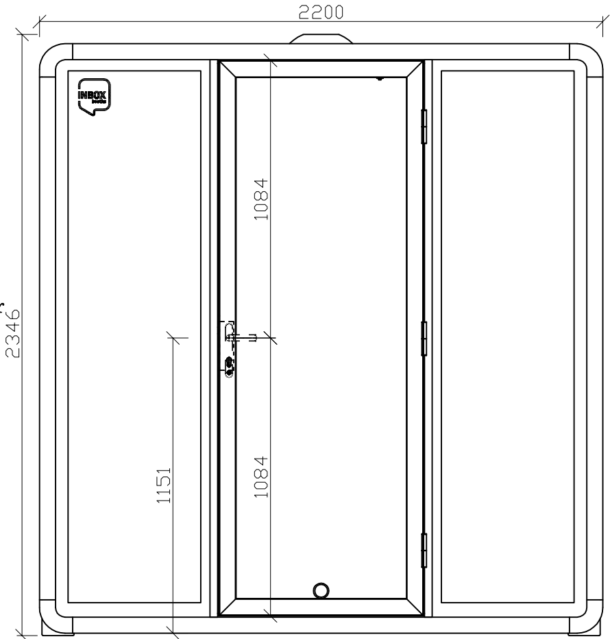
Front view
