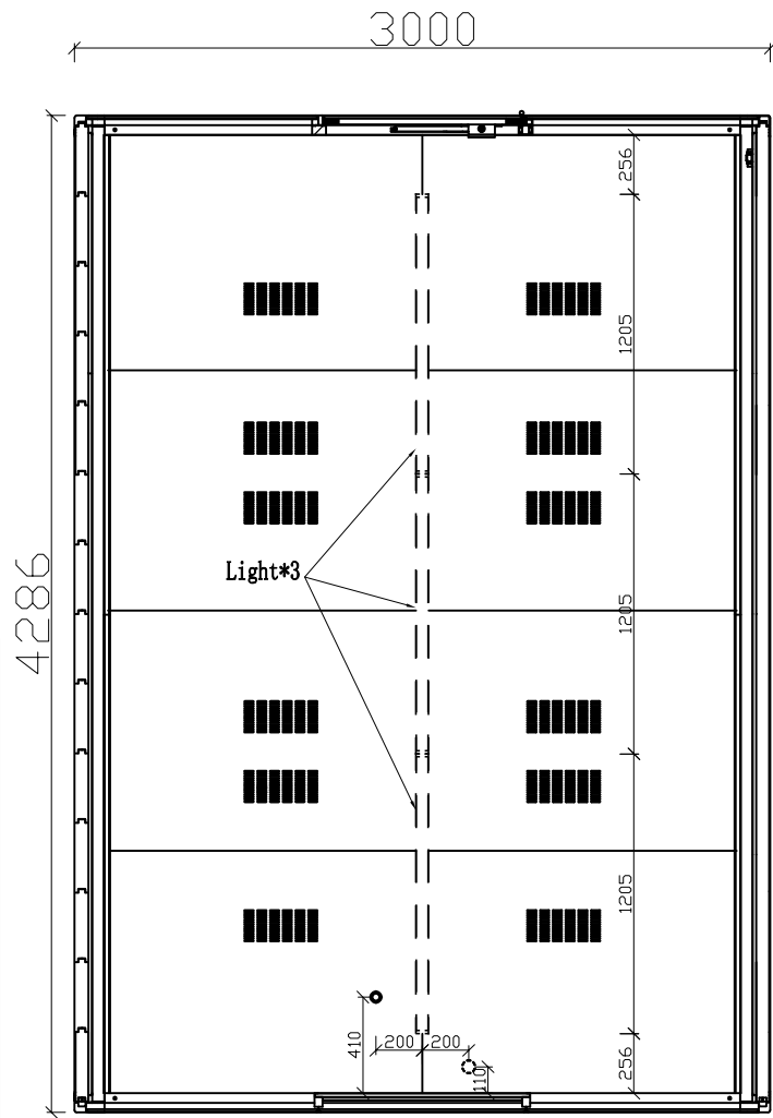
Internal top view
