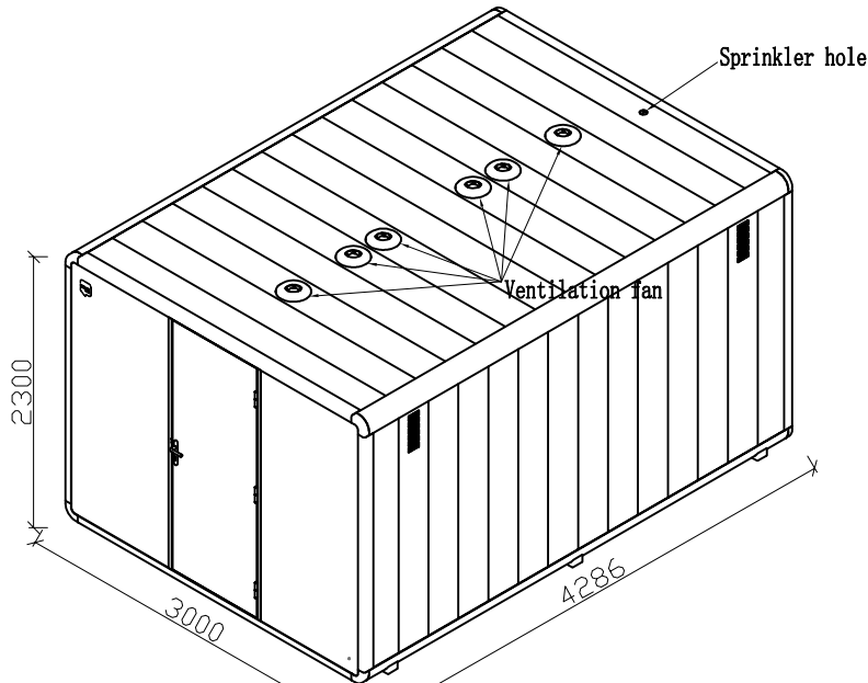
Axonometric drawing
