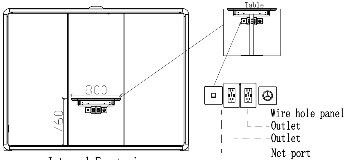
Internal Front view
