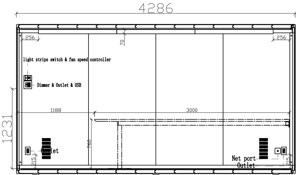
Left Inner View
